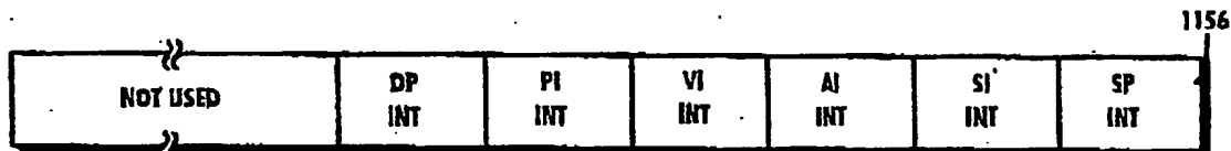
Fig. 39C INTERRUPT REGISTER (R)
